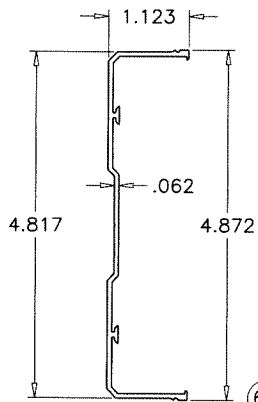
⑥A MULLION PRESSURE CAP
