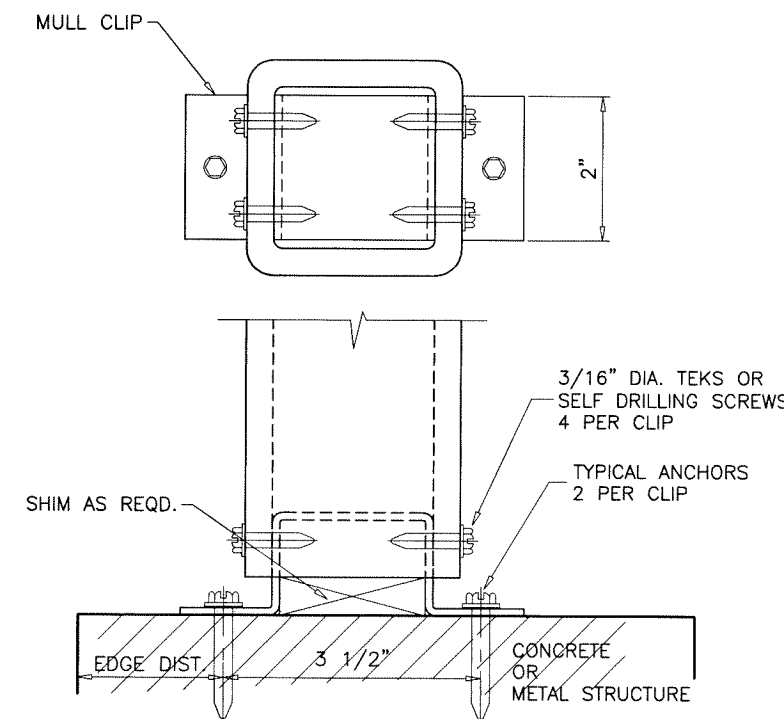
MULLION CONNECTION TYP. AT TOP AND BOTTOM
