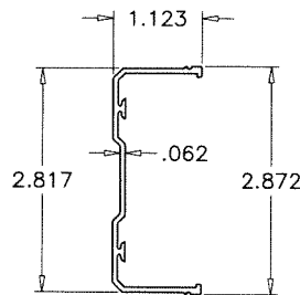
⑥ FRAME PRESSURE CAP
