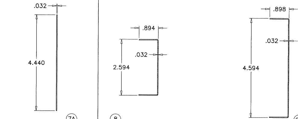
⑧ FRAME RETAINER CHANNEL
