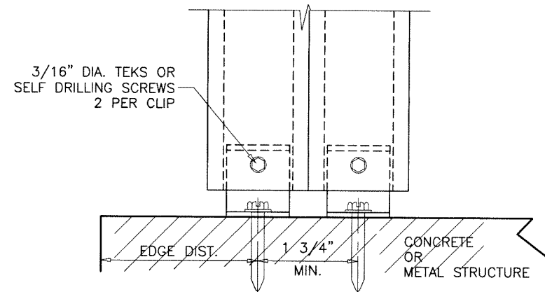
MULLION CONNECTION TYP. AT TOP AND BOTTOM
