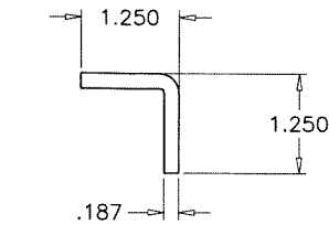
① INSTALLATION ANGLE
