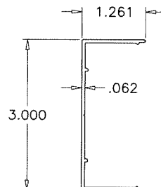
⑩ FRAME SNAP ON COVER (VERTICAL)
